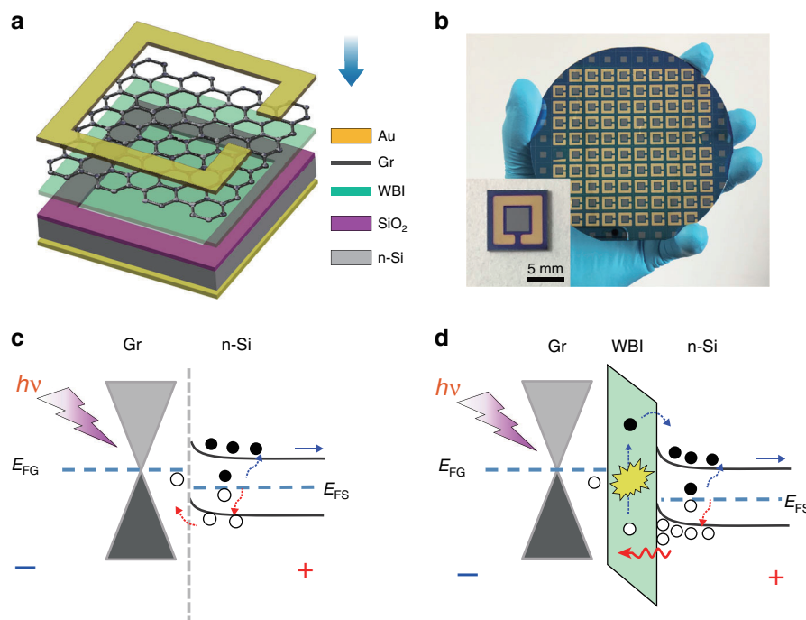
Fig. 1 Device structure and proposed working mechanism for the devices. a Schematic and b photo image of the fabricated wafer-scale graphene/insulator/Si (GIS) heterojunction photodetectors. The device size was 8 \times 8 \text{ mm}^2 with a center active region of 3 \times 3 \text{ mm}^2 . c , d Shows the corresponding energy band diagram of the conventional GS heterojunction photodetector and the GIS heterojunction photodetector under reverse bias and illumination, respectively.
